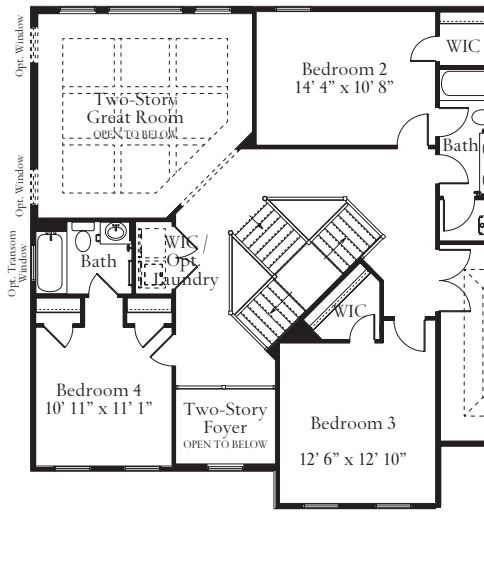
Partial alternate upper level with opt. two-story great room
