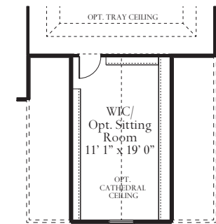
Partial upper level with opt. 3-car side load garage
